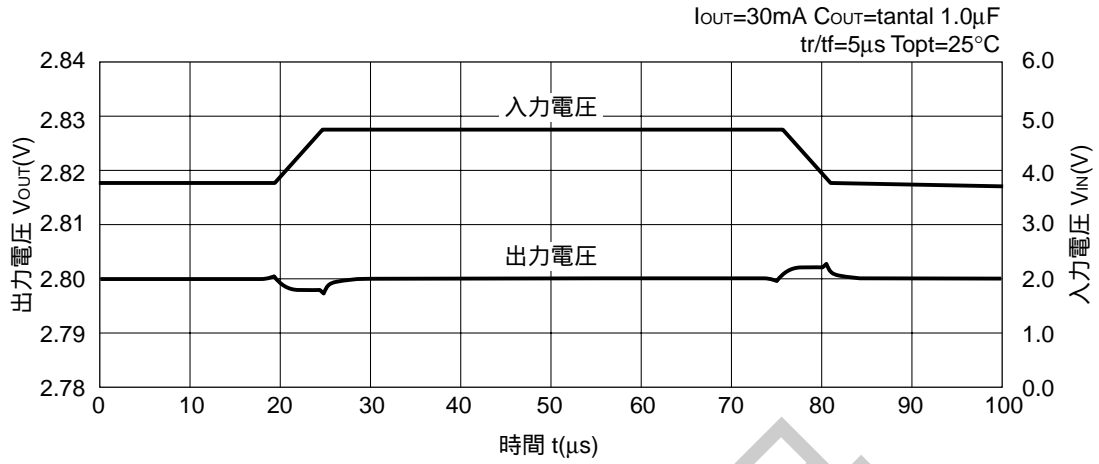
R5322N001x (2.8V, VR1)
