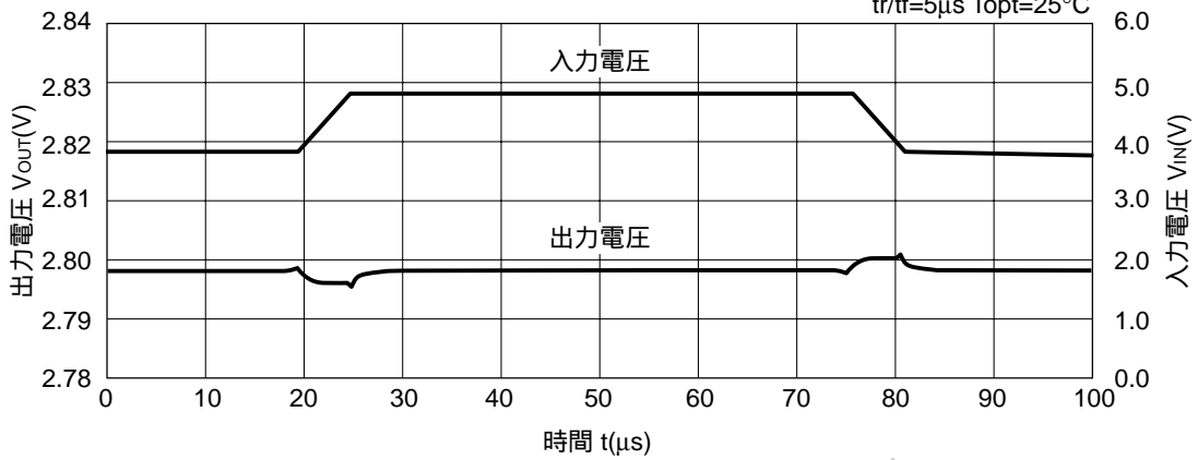
R5322N001x (2.8V, VR2)
