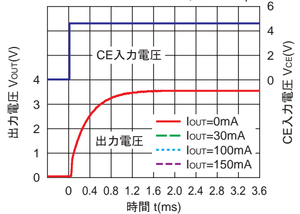
R1183Z361x
