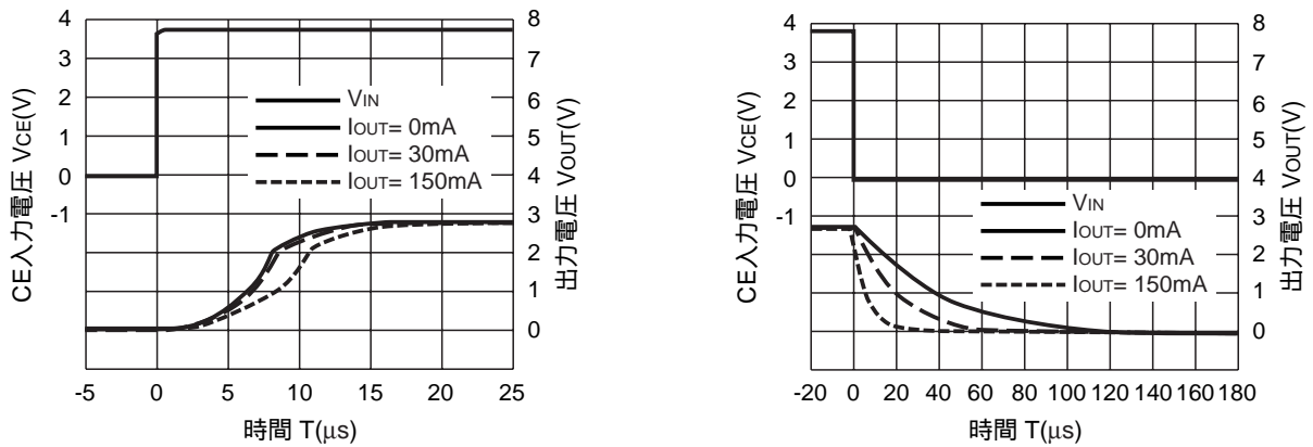
R1124N281D ( V_{IN}=3.8V , C_{IN}=\text{Ceramic } 0.47\mu A , C_{OUT}=\text{Ceramic } 0.47\mu F )
