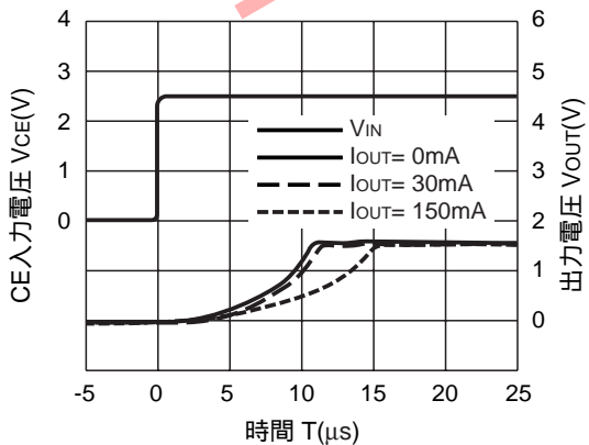
R1124N151D (VIN=2.5V, CIN=Ceramic 1.0μF, COUT=Ceramic 1.0μF)
