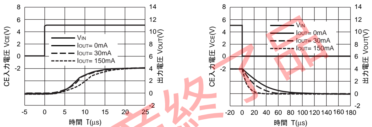
R1124N401D ( V_{IN}=5.0V , C_{IN}=\text{Ceramic } 0.47\mu A , C_{OUT}=\text{Ceramic } 0.47\mu F )
