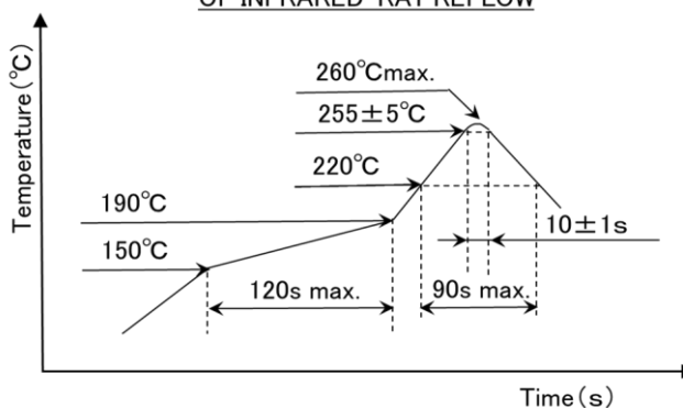
HEATING TREATMENT CONDITION OF INFRARED-RAY REFLOW
