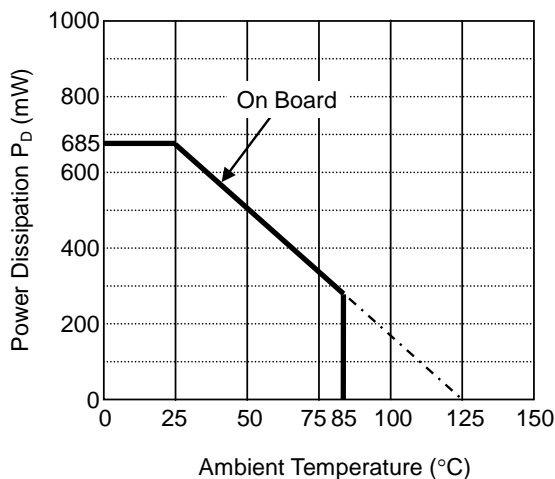
Power Dissipation
