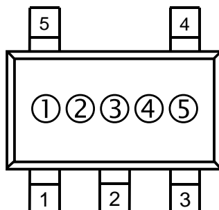
SOT-23-5 Marking Part Markings
