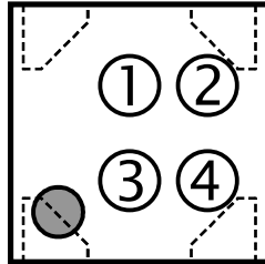
DFN(PLP)1010-4B Marking Part Markings
