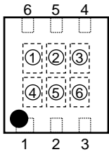
RP132Kxx1B Series
