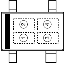
RP130Qxx1A Series
