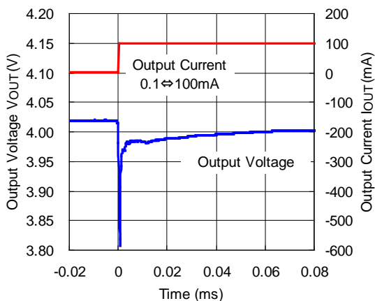
RP202x40xx (Auto ECO Low Power Mode⇒FAST Mode) VIN=5.0V
