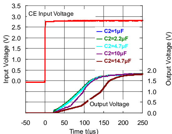
RP202x18xx VIN=2.8V, IOUT=0mA
