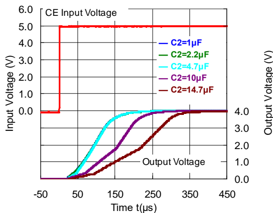
RP202x40xx VIN=5.0V, IOUT=0mA
