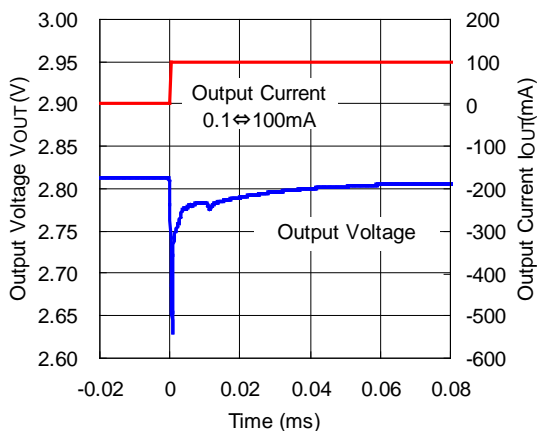
RP202x28xx (Auto ECO Low Power Mode⇒FAST Mode) VIN=3.8V
