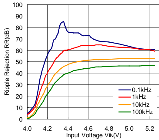
RP202x40xx (Auto ECO FAST Mode)
