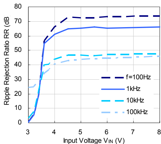
R1511x030B/R1511x001C (I OUT =100mA)
