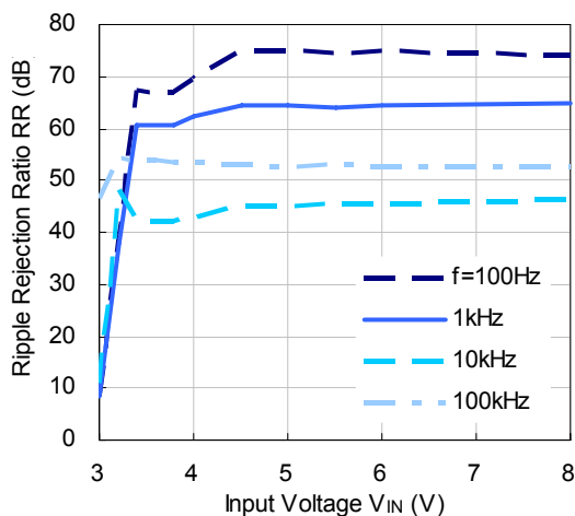
R1511x030B/R1511x001C (I OUT =1mA)
