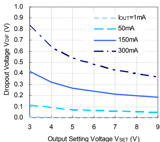
6) Dropout Voltage Vs. Setting Voltage (Ta=25°C)
