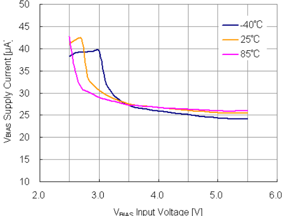
V BIAS Supply Current vs. V BIAS Input Voltage
