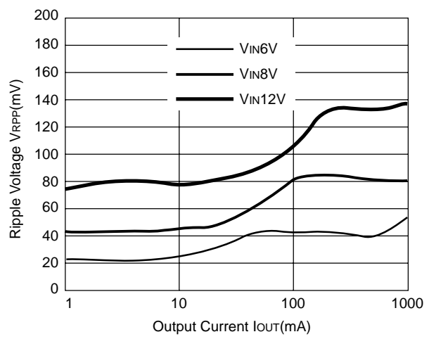
R1223N502A L=27μH
