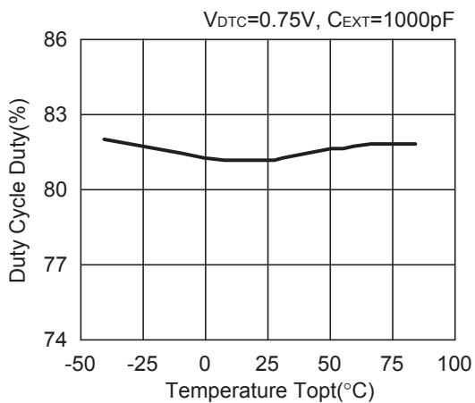
R1212D100A
