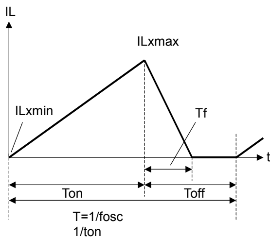
Discontinuous Mode
