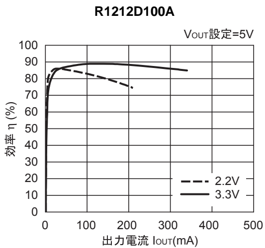
R1212D100A
