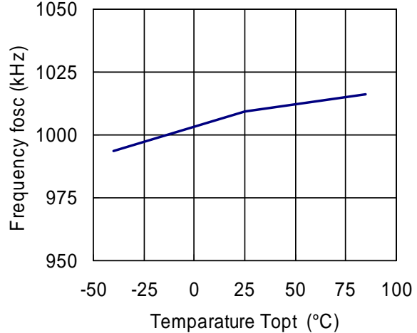
10) Oscillator Frequency vs. Temperature (f osc =1.0MHz)
