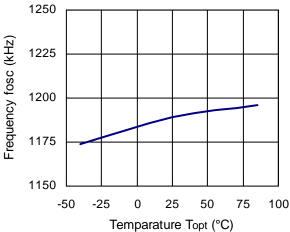
9) Oscillator Frequency vs. Temperature (f osc =1.2MHz)
